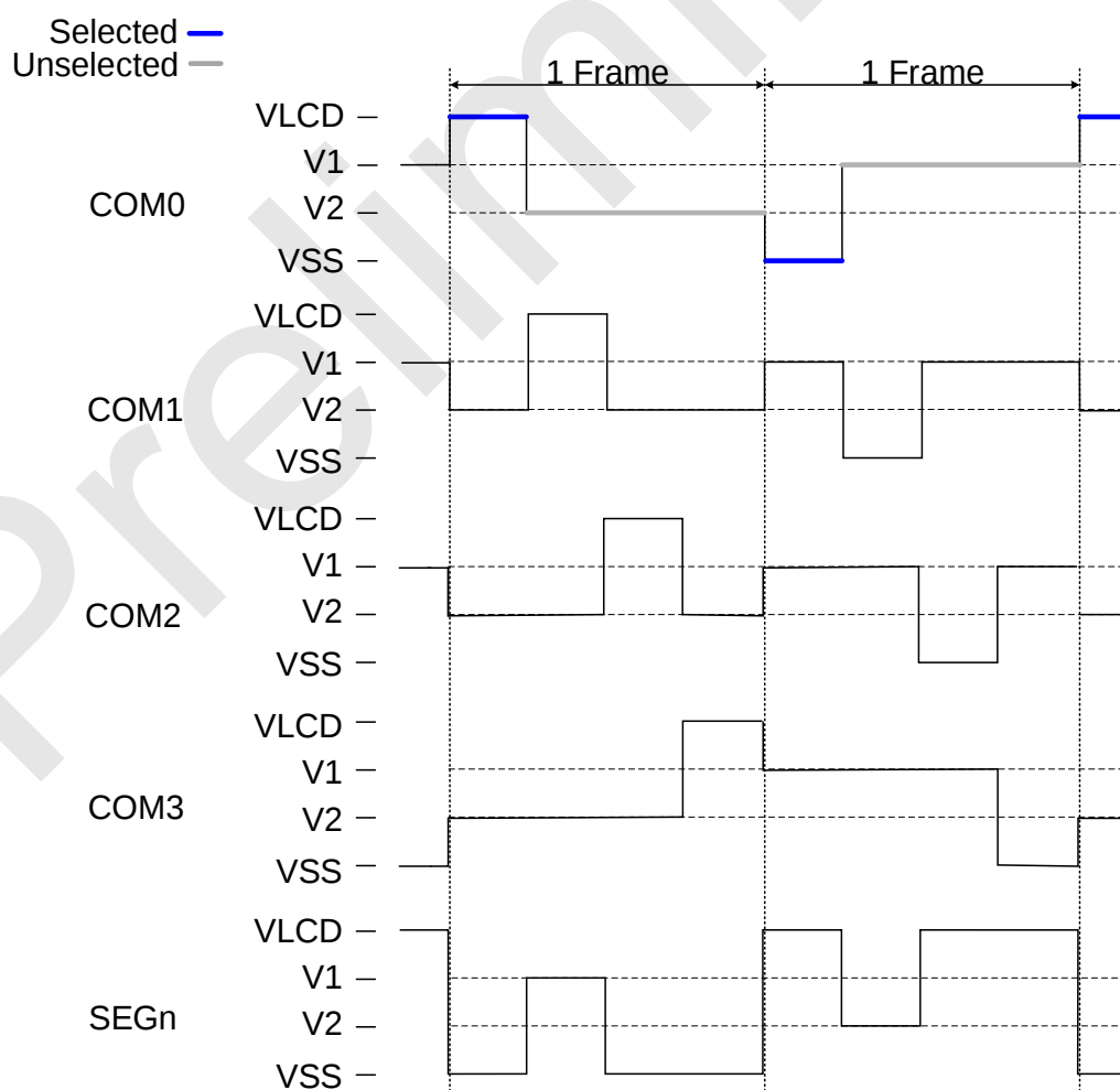
1/3 Bias LCD 选通和非选通电压
