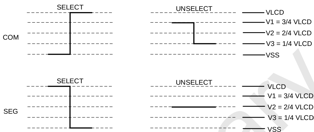
1/4 Bias LCD 选通和非选通电压
